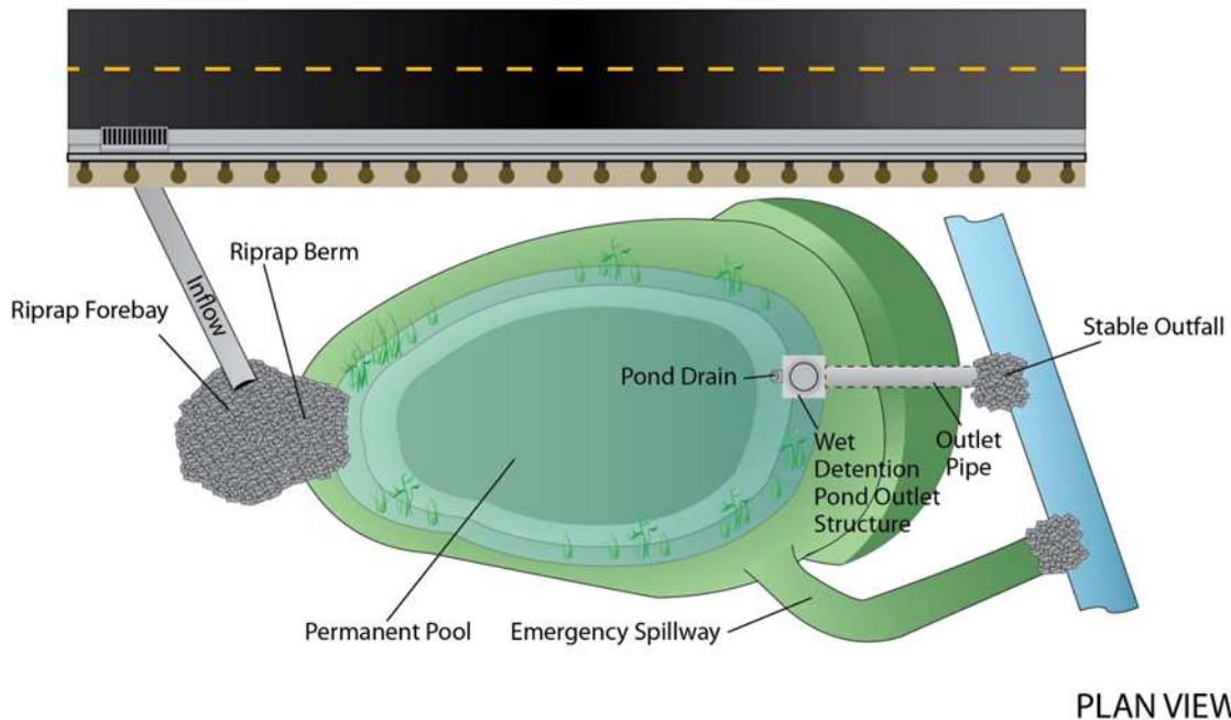
Figure 10.6.9-1 - Typical wet detention pond configuration
