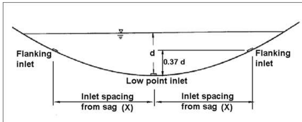
Figure 6.14 - Flanking inlet schematic
