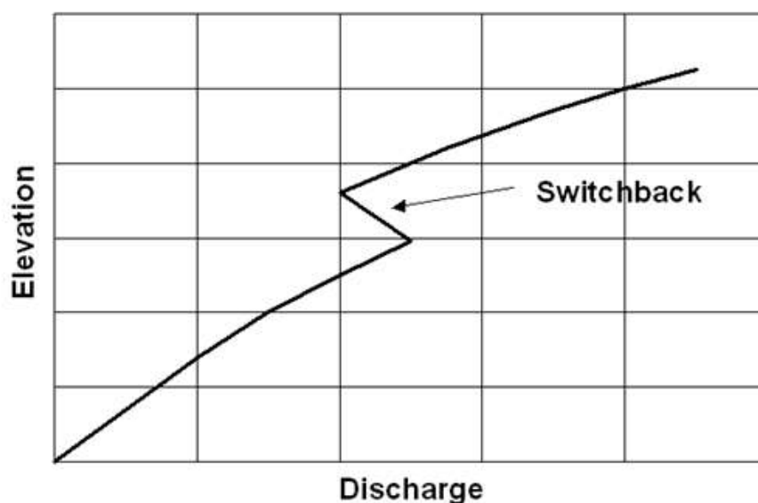
Figure 5.4 - Switchback phenomenon
