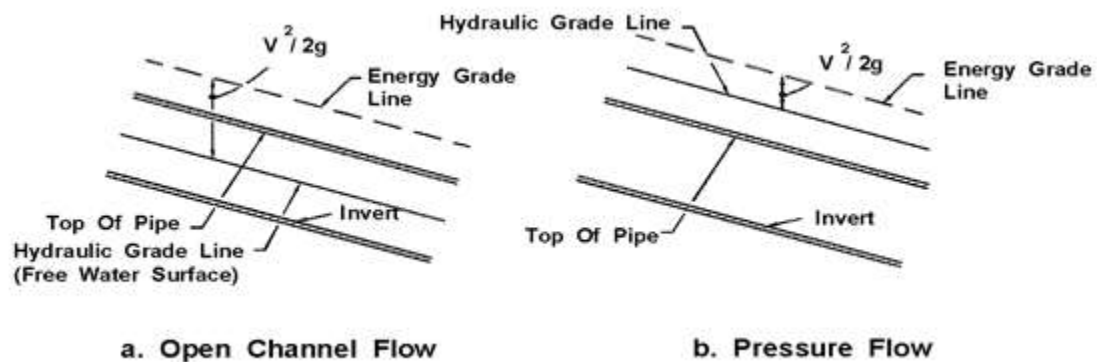
Figure 7.5 - Hydraulic and energy grade lines in pipe flow
