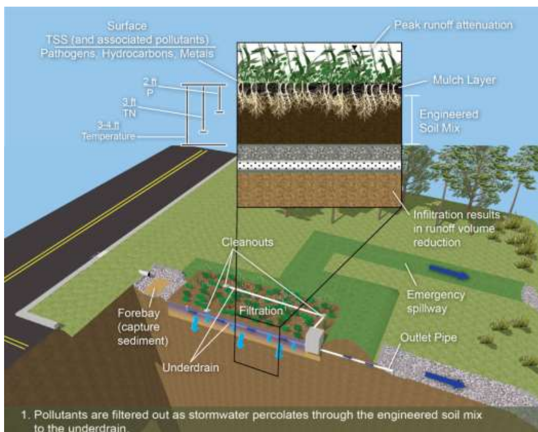
Figure 10.6.7-2 - Typical bioretention basin components and treatment processes, and pollutant removal zones (10-26)
