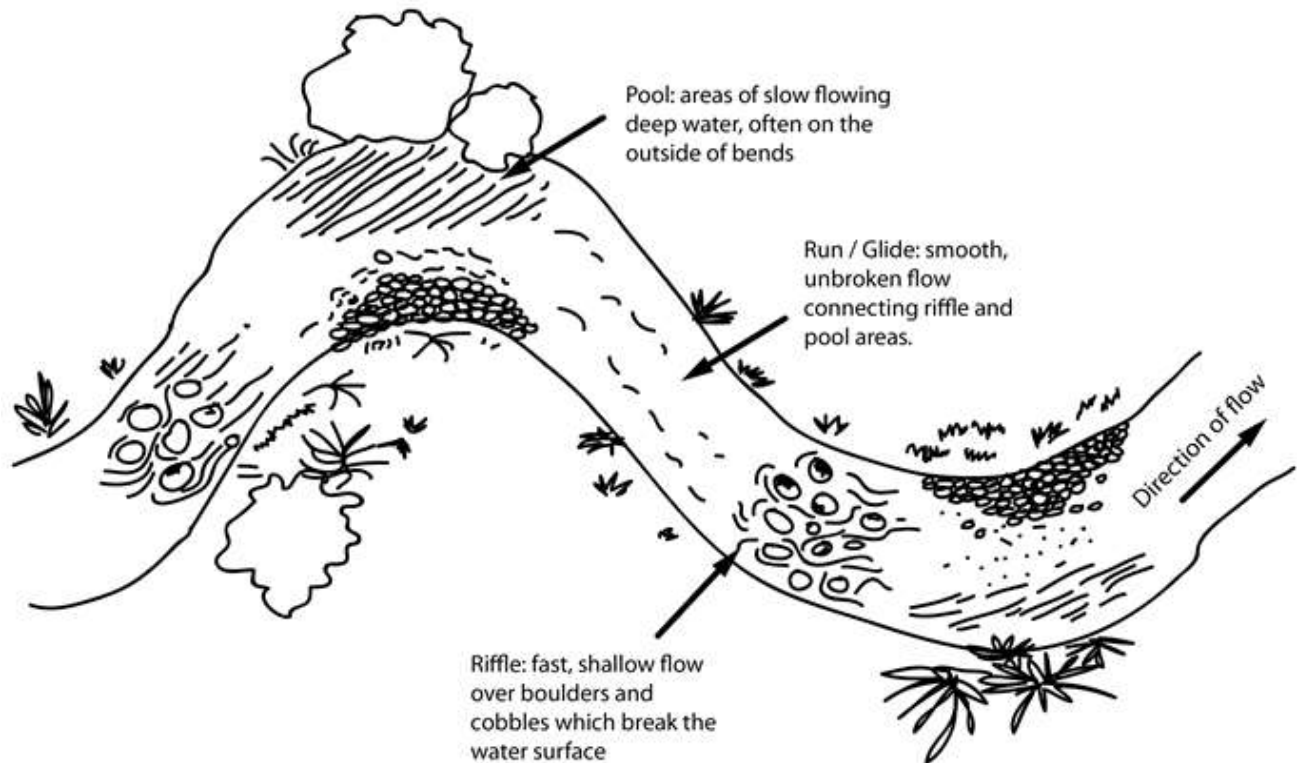
Figure 11.2 - The Stream Reach
