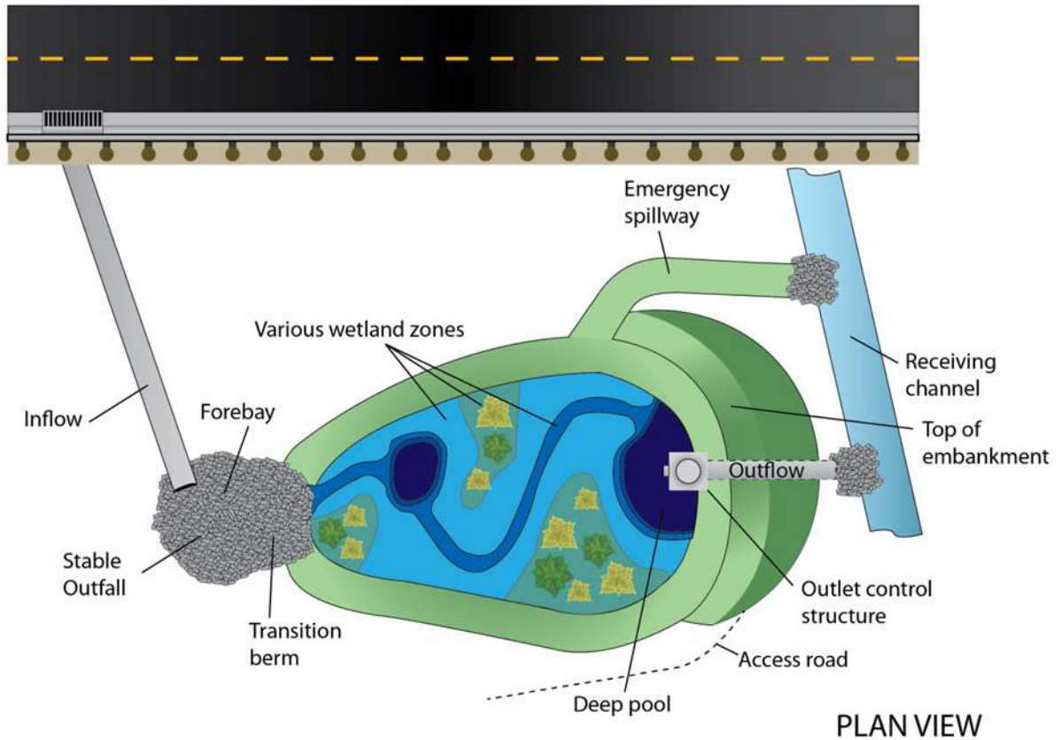
Figure 10.6.10-1 - Typical Level 1 stormwater wetland configuration
