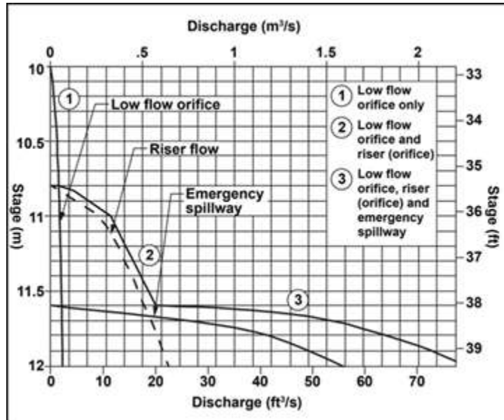
Figure 10.7-7 - Typical combined stage-discharge relationship (10-7)
