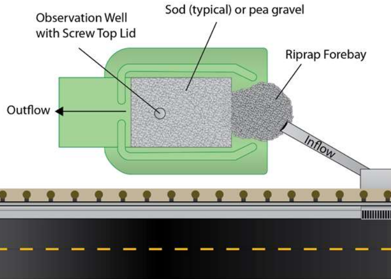
Figure 10.6.4-2 - Typical infiltration trench – plan and profile views
