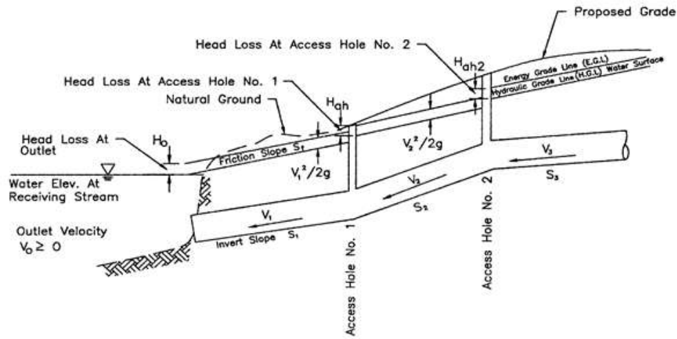
Figure 7.12 - Energy and hydraulic grade line illustration
