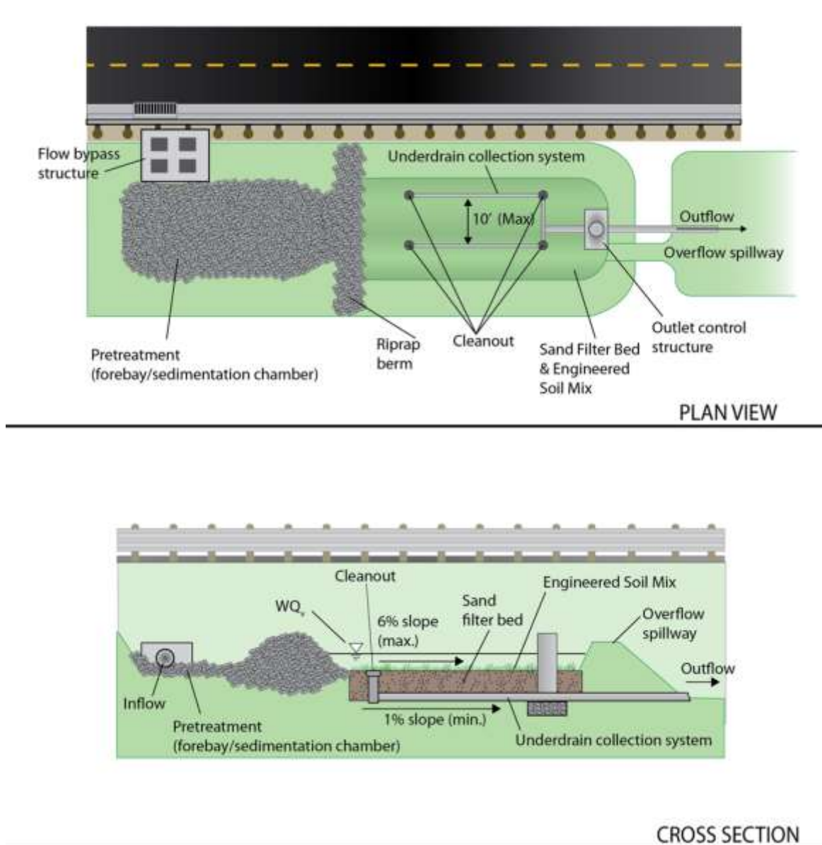
Figure 10.6.6-3 - Surface sand filter
