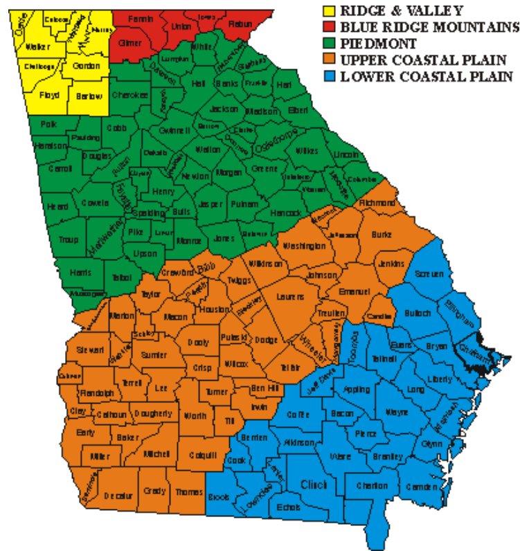
Figure 10.2-1 - Physiographic Regions of Georgia Reference: Georgia Department of Natural Resources
