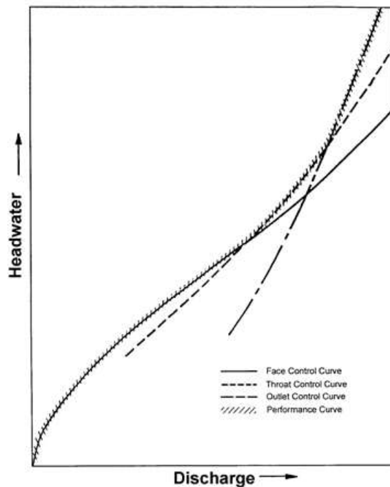
Figure 8.12 - Schematic of culvert performance curve with improved inlet
