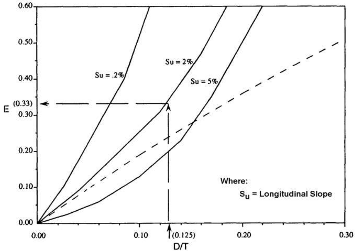
Figure 13.5 - Efficiency curves for circular scuppers (13-2)
