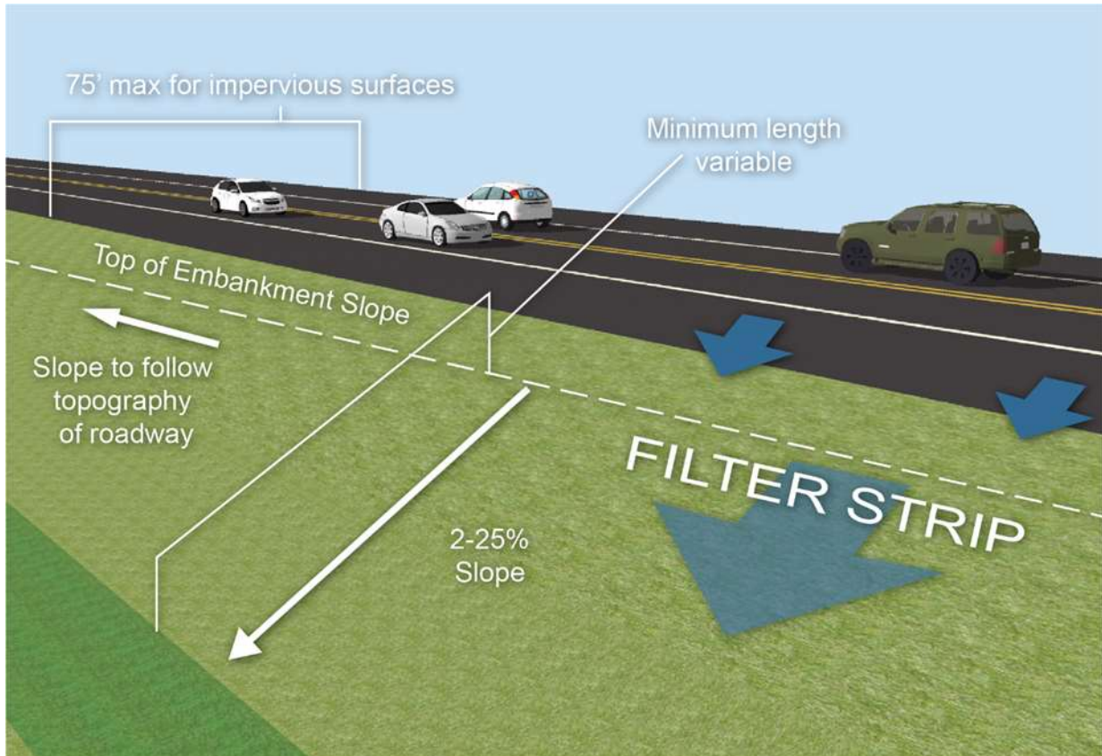
Figure 10.6.1-3 - Typical filter strip design for a roadway application
