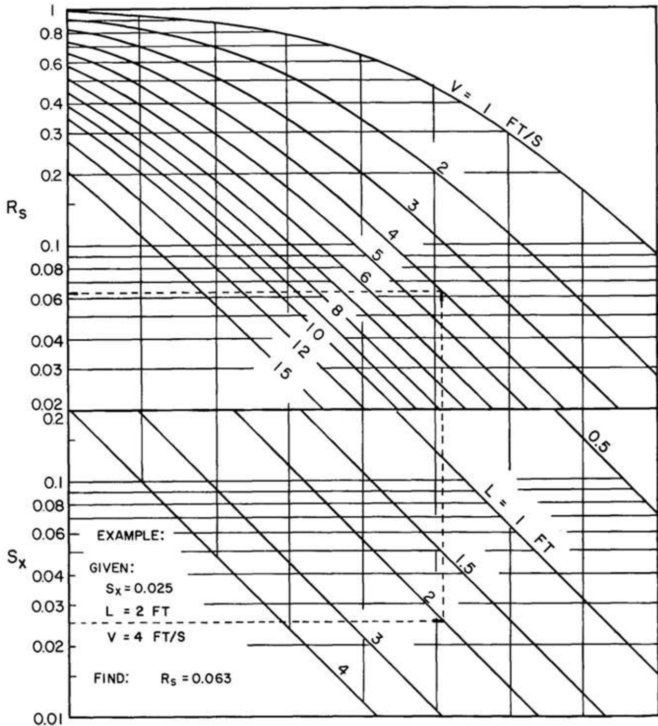
Grate Inlet Side Flow Intercept Efficiency
