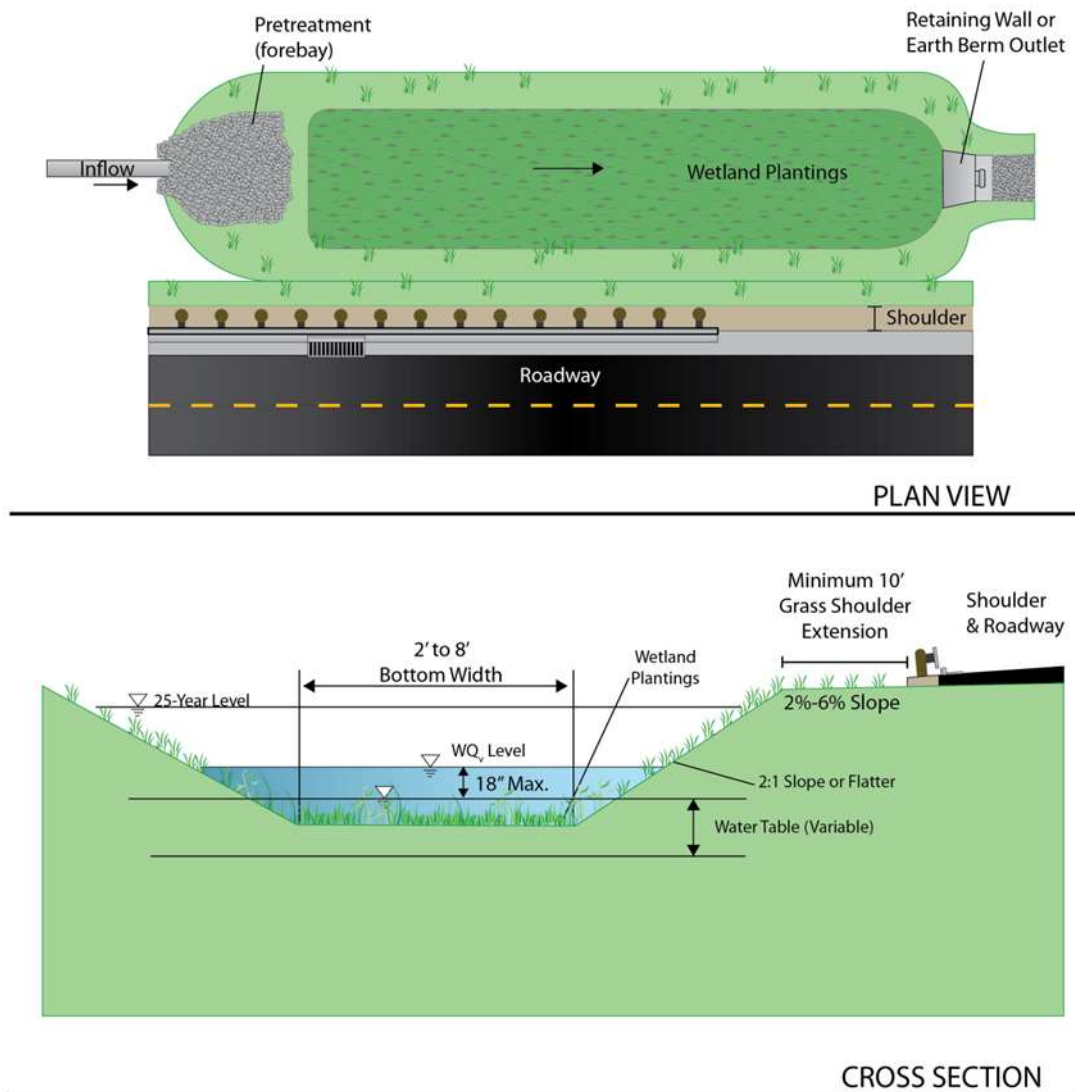
Figure 10.6.3-4 - Enhanced wet swale schematic
