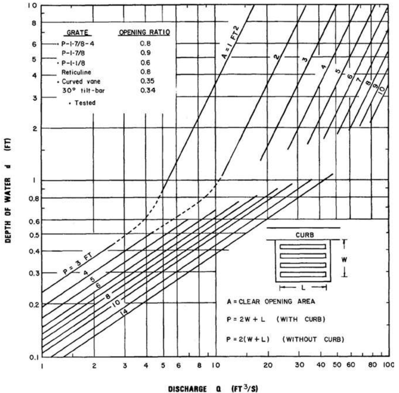
Chart 6.3 - Source: HEC 22 (6-4)
