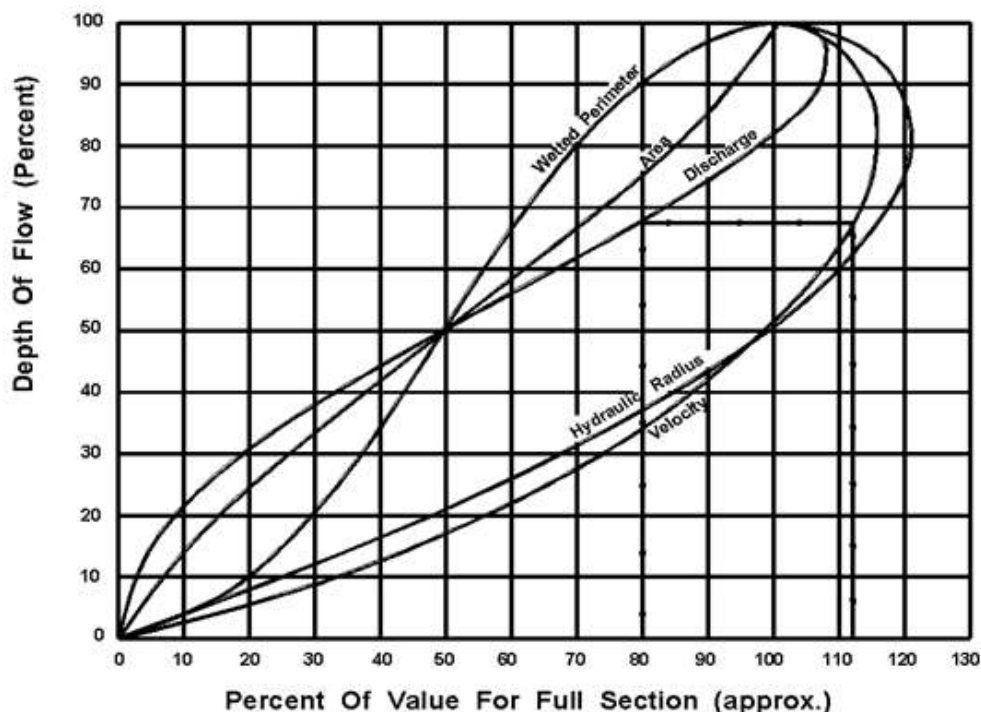
Figure 7.1 - Hydraulics elements chart
