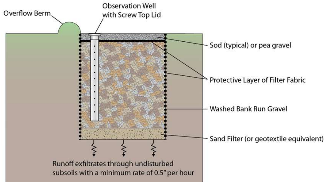
CROSS SECTION
