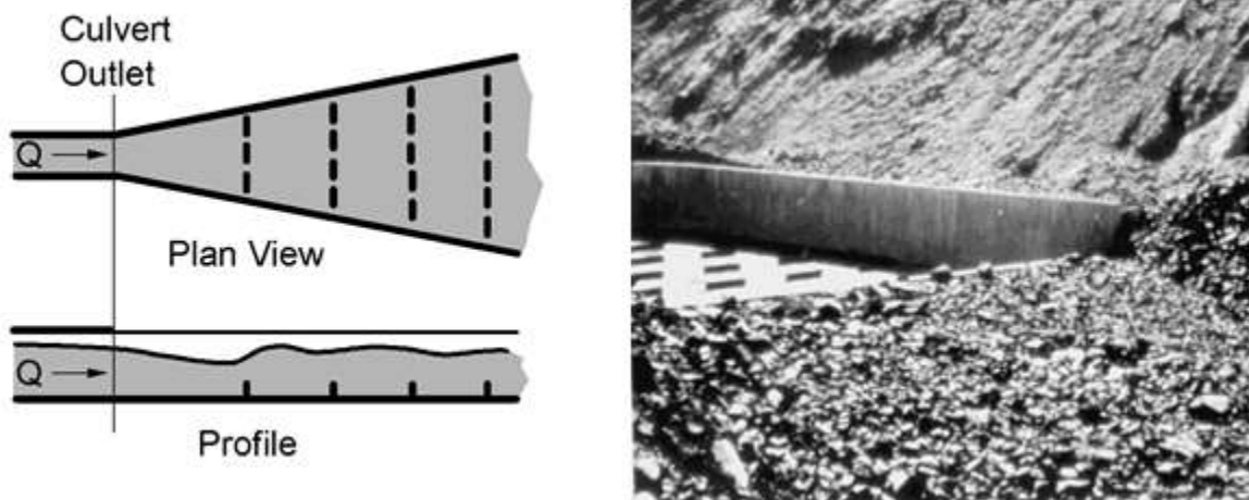
Figure 8.19b (right) - Photo of CSU rigid boundary basin
