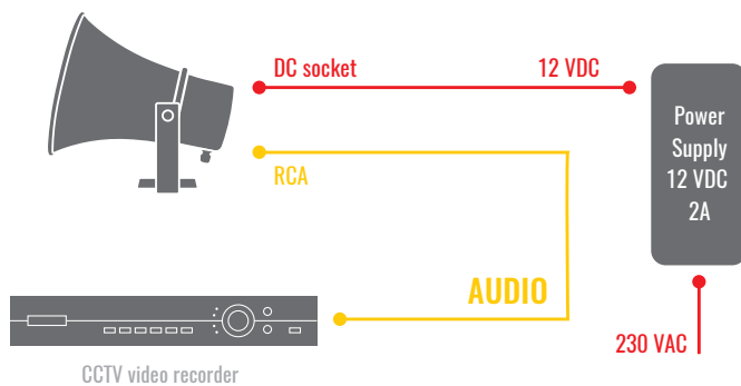
Wiring diagram
