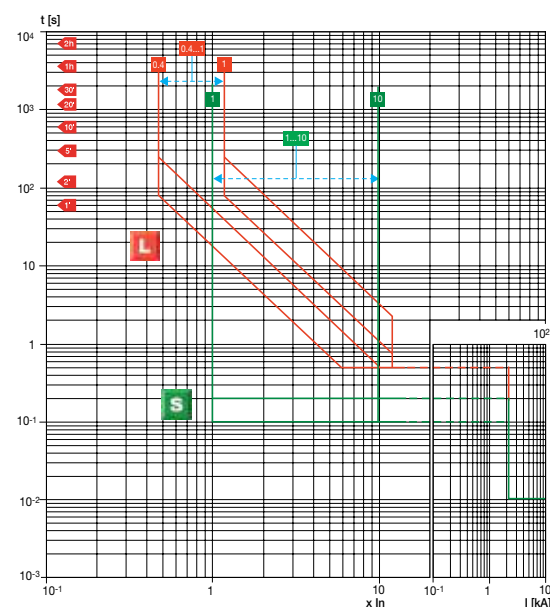
XT2 Ekip LS/I L-S functions
