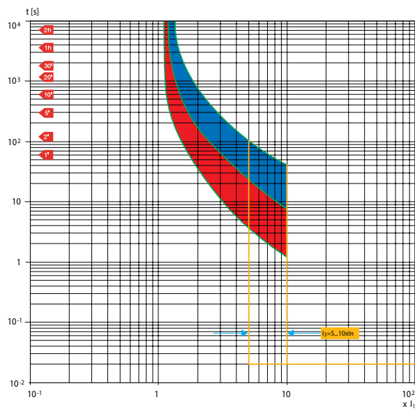
XT6 800 TMA In=630A
