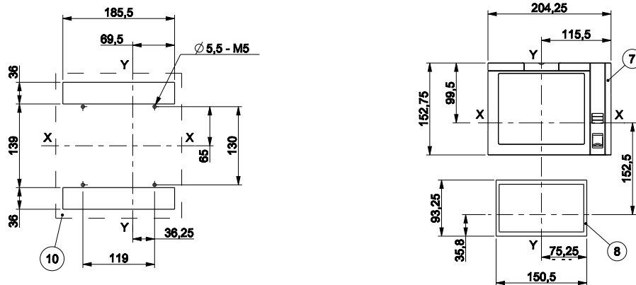
Drilling template for support sheet Flange
