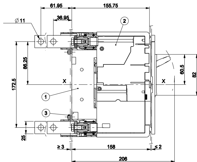
Terminals VR
