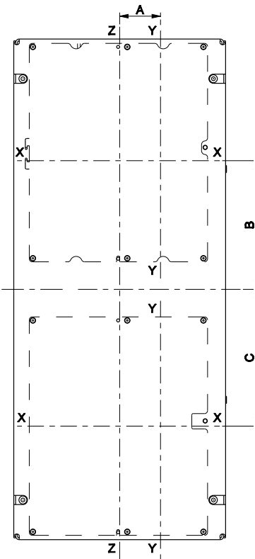
Interlocking plate
