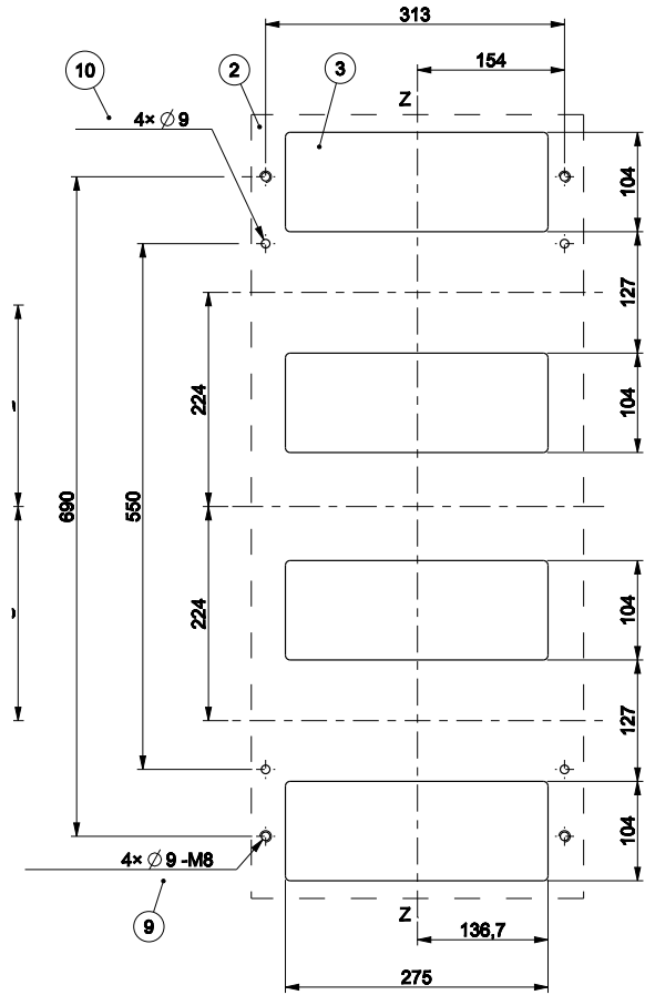
Drilling template
