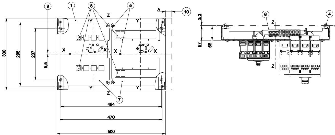
Drilling template
