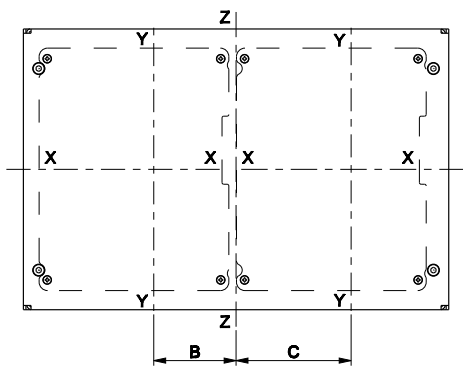
Interlocking plate
