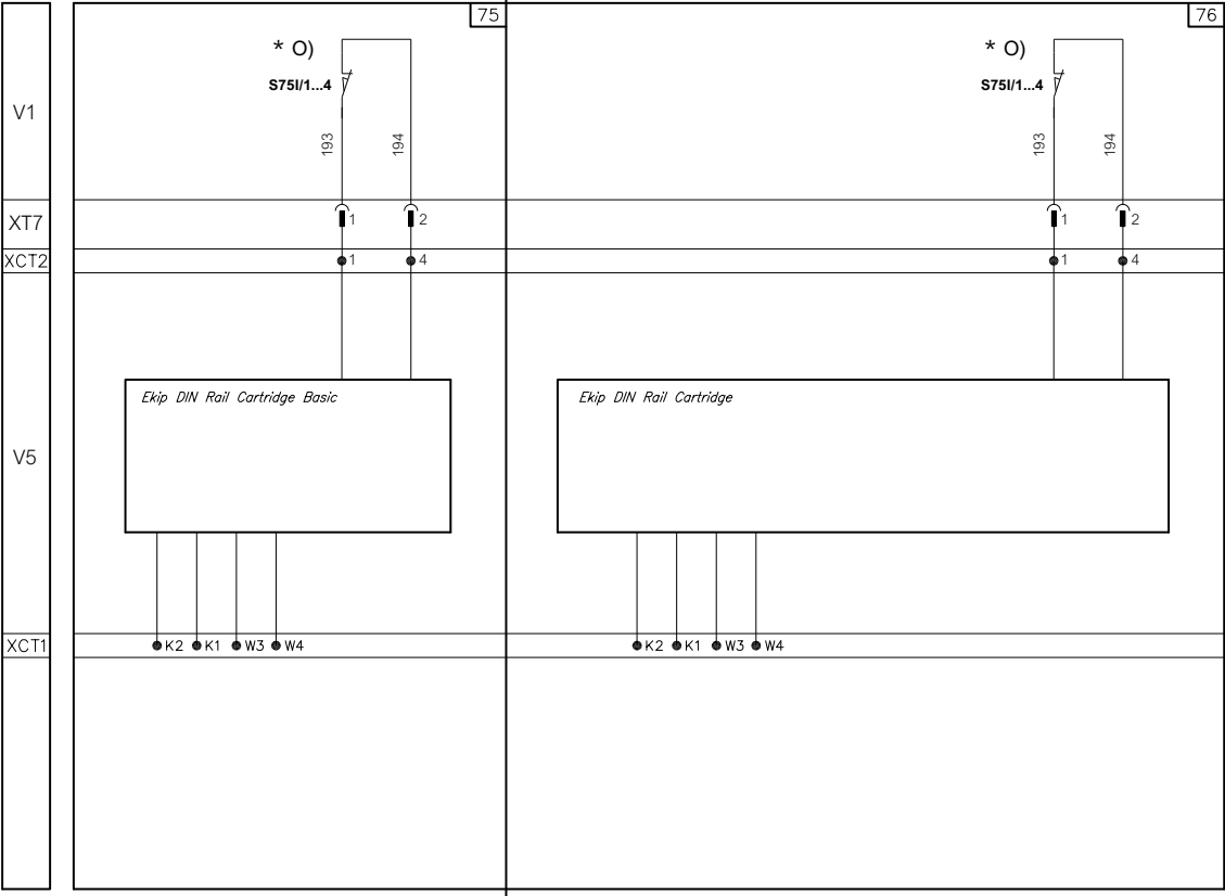
75a) Ekip Cartridge for one module and one Ekip Supply 76a) Ekip Cartridge for three modules and one Ekip Supply
