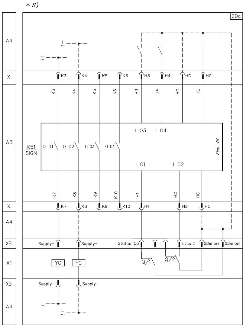
20C) Ekip 4k on Ekip UP protect, protect+, and control+ version with YO and YC command and 2 status input
