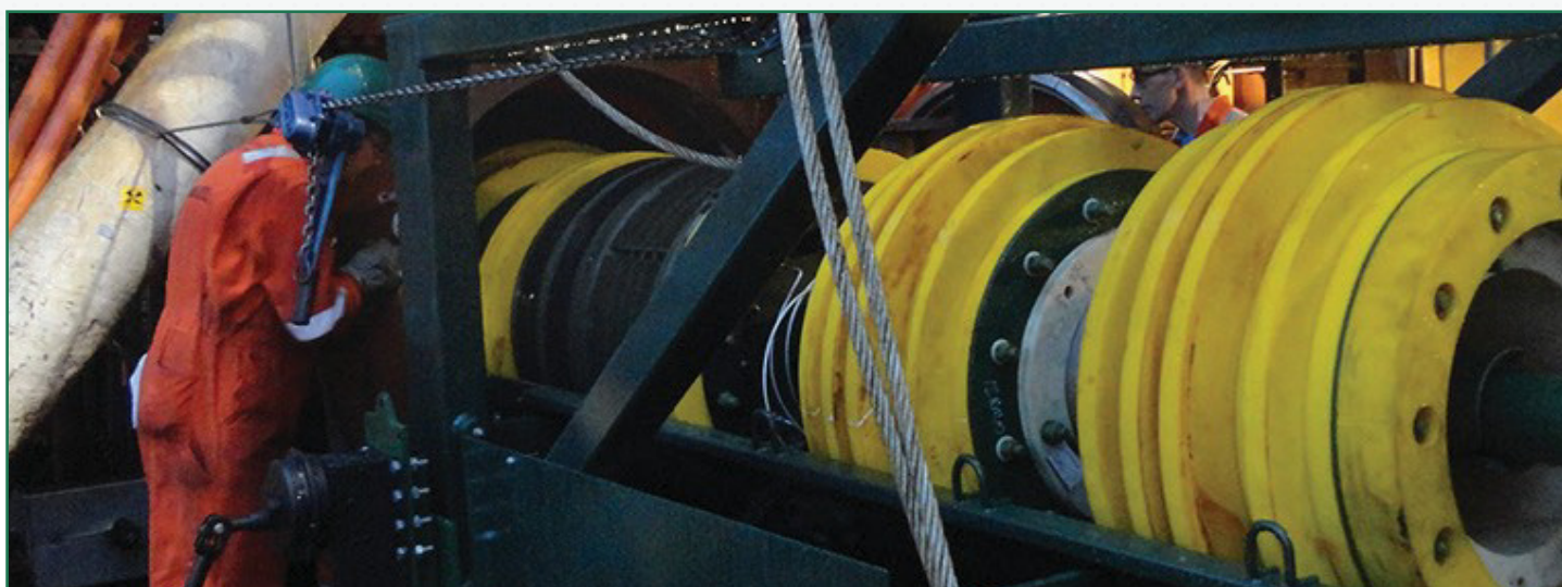
36" Remote Tecno Plug being deployed into pipeline launcher
