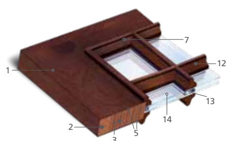
Patio Door Panel Design
