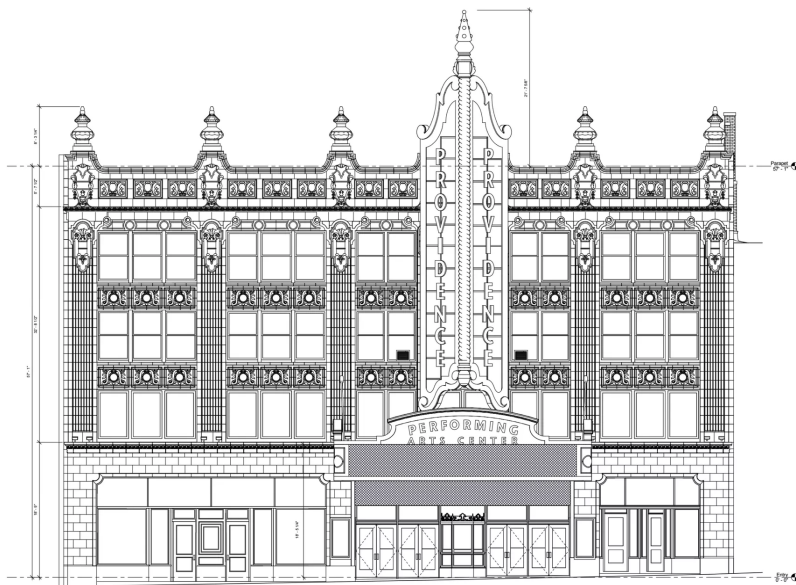
View of 3D BIM Model and Exterior Elevation – Providence Performing Arts Center, Providence, RI
