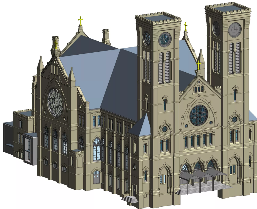
3D BIM Documentation of The Cathedral of Saints Peter and Paul - Providence, Rhode Island
