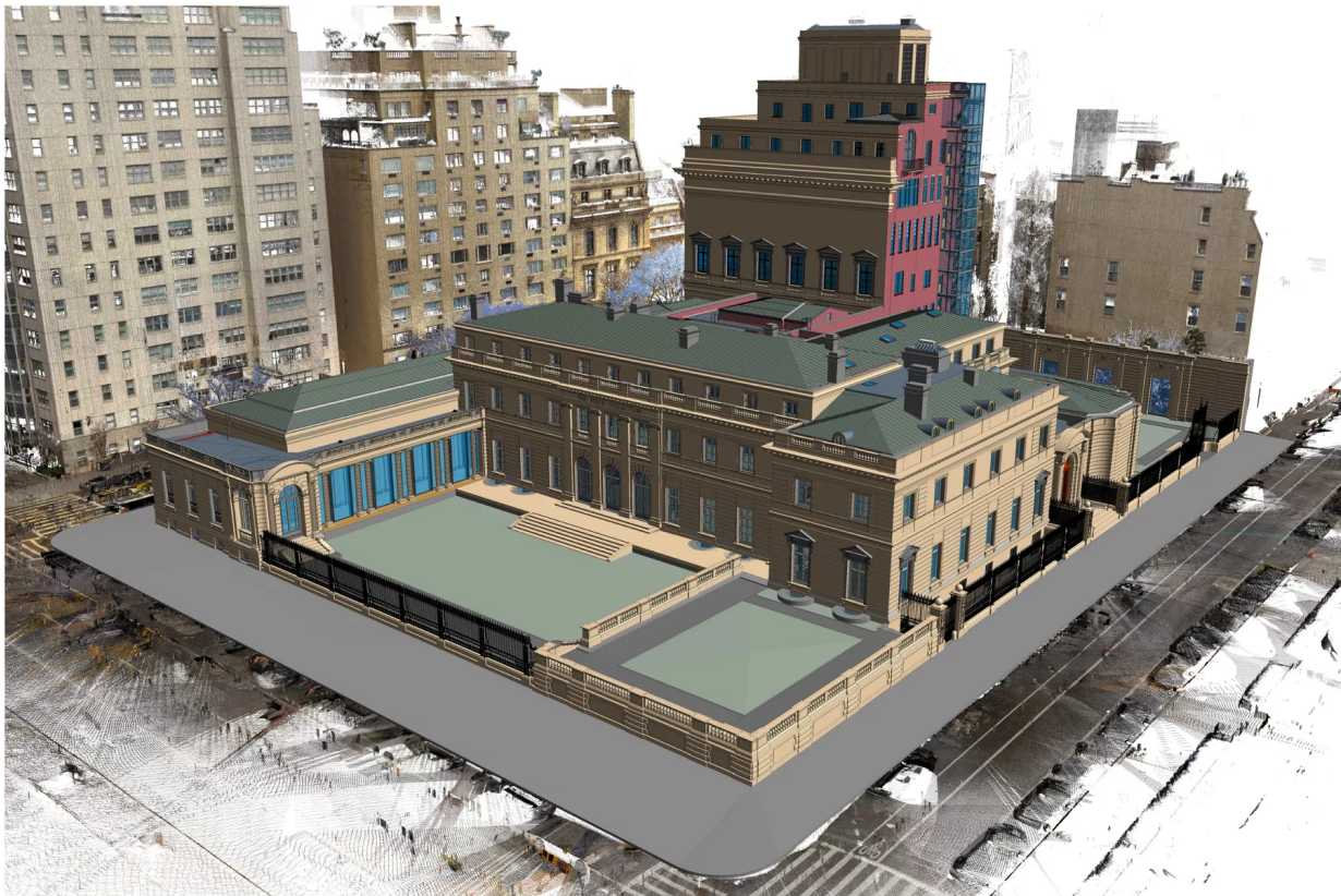
3D Building Information Model and Scan Data - The Frick Collection, New York, NY
