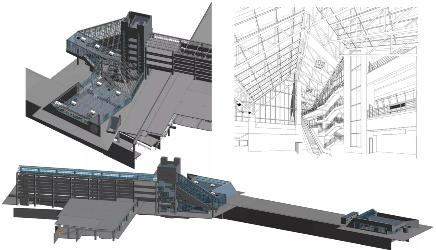
3D BIM of MBTA Alewife Station - Cambridge, Massachusetts
