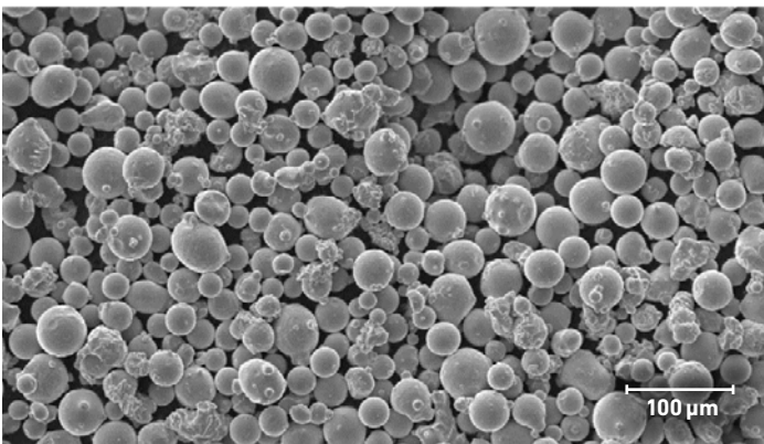
FIGURE 1 — SEM IMAGE OF TYPICAL POWDER RANGE X POWDER
