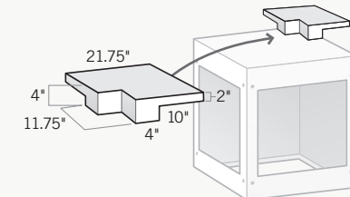
Corner Raised Backsplash Creates a 4" high raised corner backsplash with a 10" cantilever; connects to straight raised backsplash for L-shaped configurations. Requires 2 bolts for mounting (not included).
