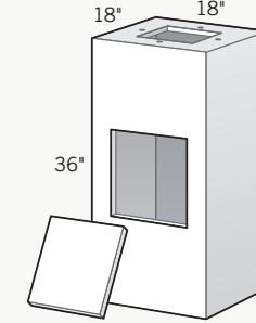
Column with End Cap 18"D × 18"L × 36"H Instantly build perfect stone or brick columns/ Column ships with access panel. Designed with top and bottom flange for attaching masonry anchor or bolting.
