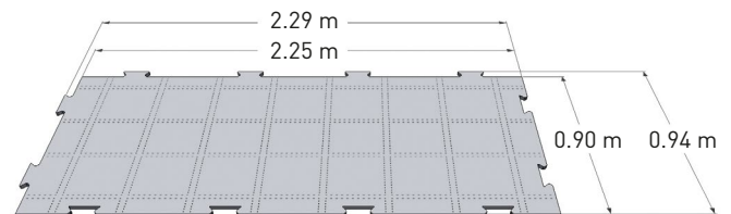
Dimensions ProPlay ® -Sport sheet
