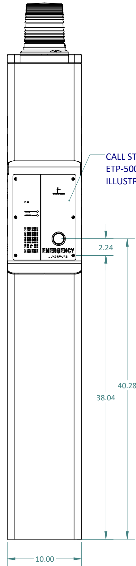
FRONT VIEW
