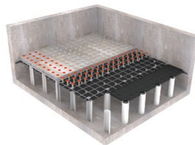
Cutaway rendering of the MULTICRETE II
