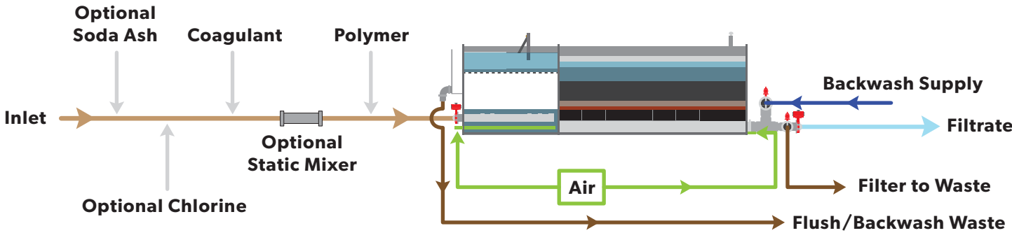
Trident Process Flow Diagram
