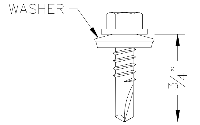
3/4" PAINTED SCREW
