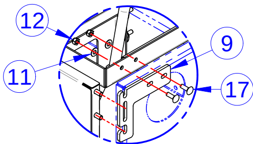
DETAIL D
