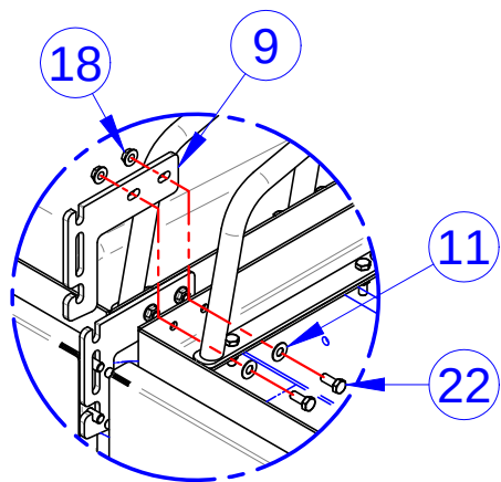
DETAIL C
