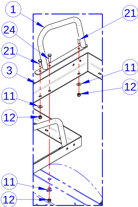
DETAIL A
