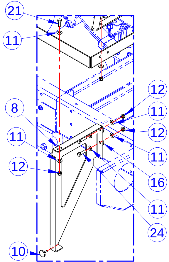
DETAIL B
