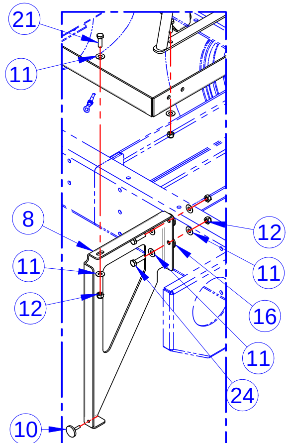
DETAIL B
