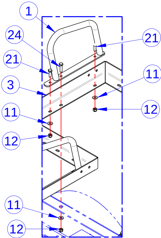
DETAIL A
