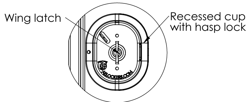
DETAIL A SCALE 1 : 4
