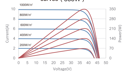
Current-Voltage & Power-Voltage curves (355W)
