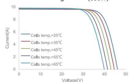
Current-Voltage curves(355W)
