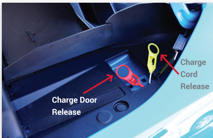
Manual Charge Door and Charging Cord Releases can be found in the cowl area for each charge port assembly
