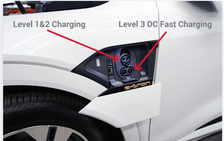
Driver Side Charge Door Level 1/2 & Level 3 DC Fast Charge Capable
