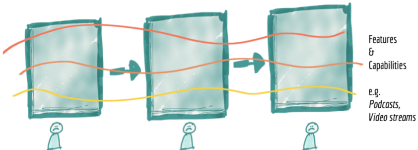
Figure 1: When you make a change to a centralized platform, you need to update each component and coordinate between several different teams. Source: Thoughtworks
