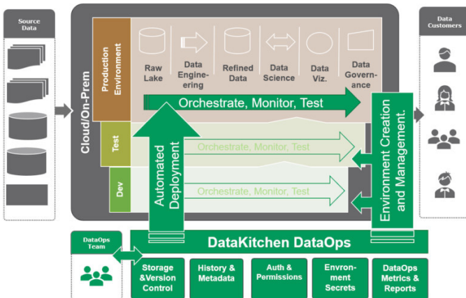
Figure 6: The DataKitchen DataOps Platform eliminates waste from the processes that manage integration, development and operation
