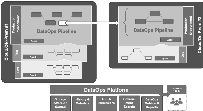
Figure 72: Multi-location DataOps Data Architecture
