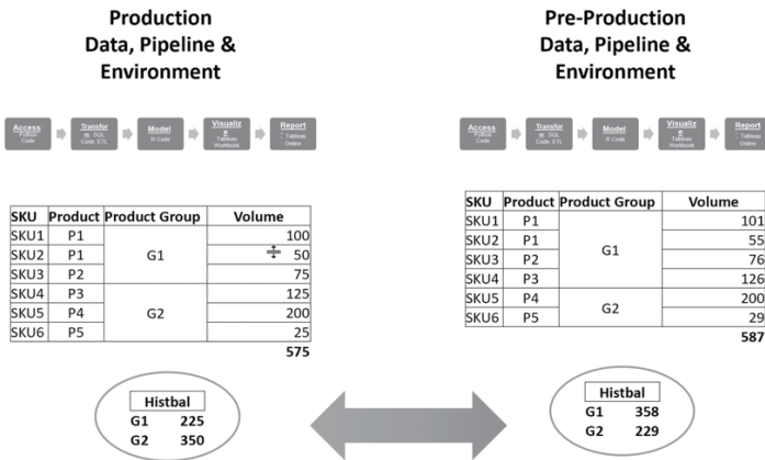
Figure 90: It's not enough for analytics to be correct. Accurate analytics that “look wrong” to users raise credibility questions.
