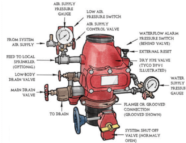
Dry Valve System
