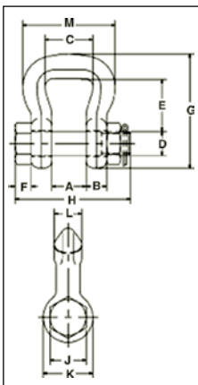
S-252 Bolt Type Sling Shackle
