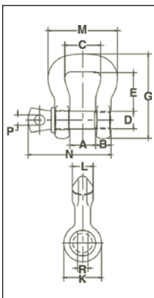
S-253 Screw Pin Sling Shackle
