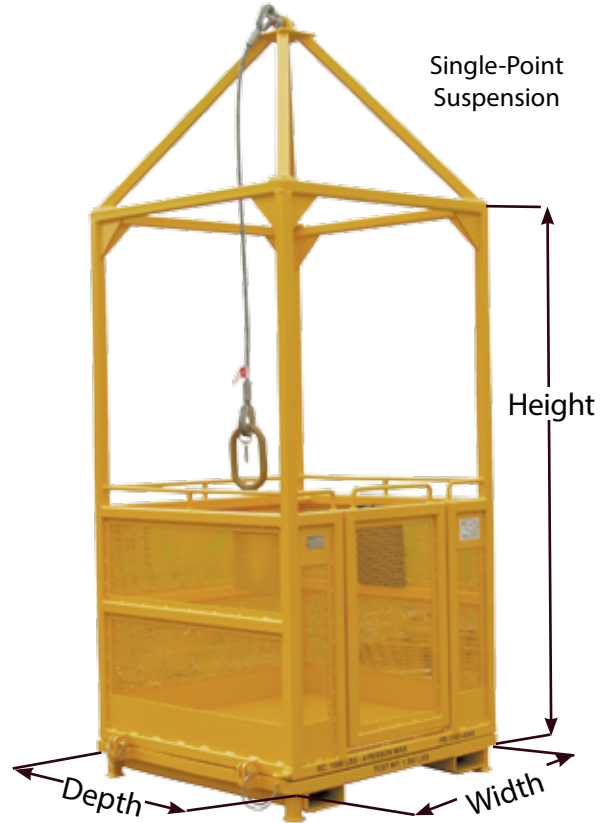
Model: PB - Liftmax® Personnel Basket PBS - Liftmax® Personnel Basket, single point suspension
