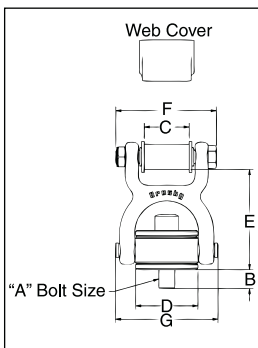
HR-125W Hoist Ring to Web
